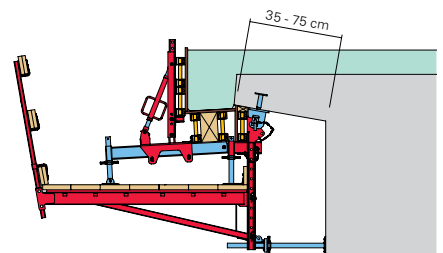
Use in the intermediate area on cantilevers between 35 and 75 cm long.
